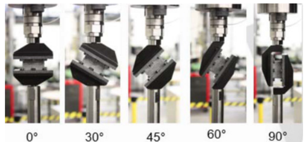
Figure 4. Dynamic Arcan devices.
