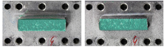
Figure 6. Cohesive failure.
