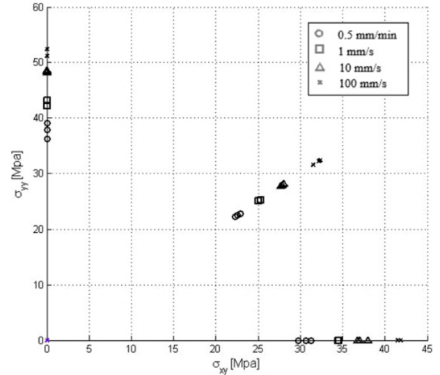
Figure 7. Failure surface.
