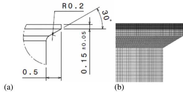
Figure 2. (a) Beak geometry, (b) Mesh of the beak.
