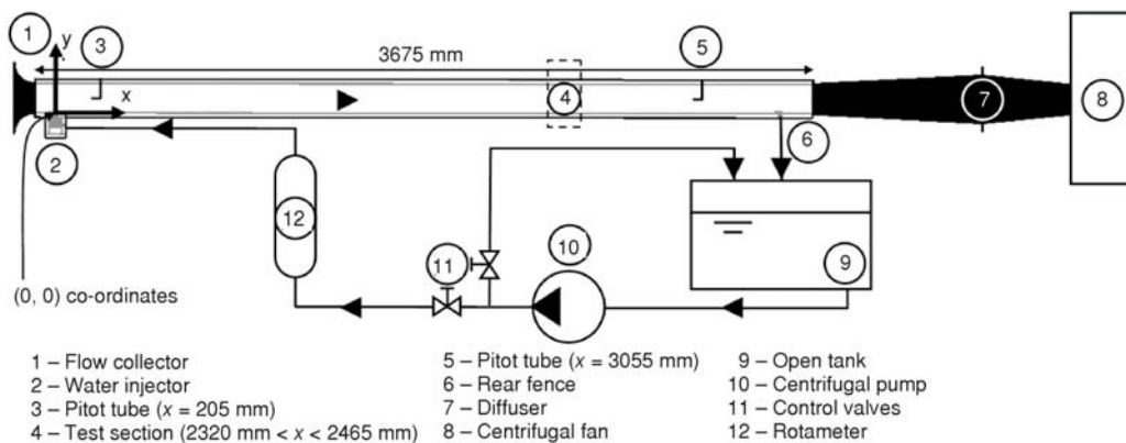
Figure 1. Experimental apparatus
